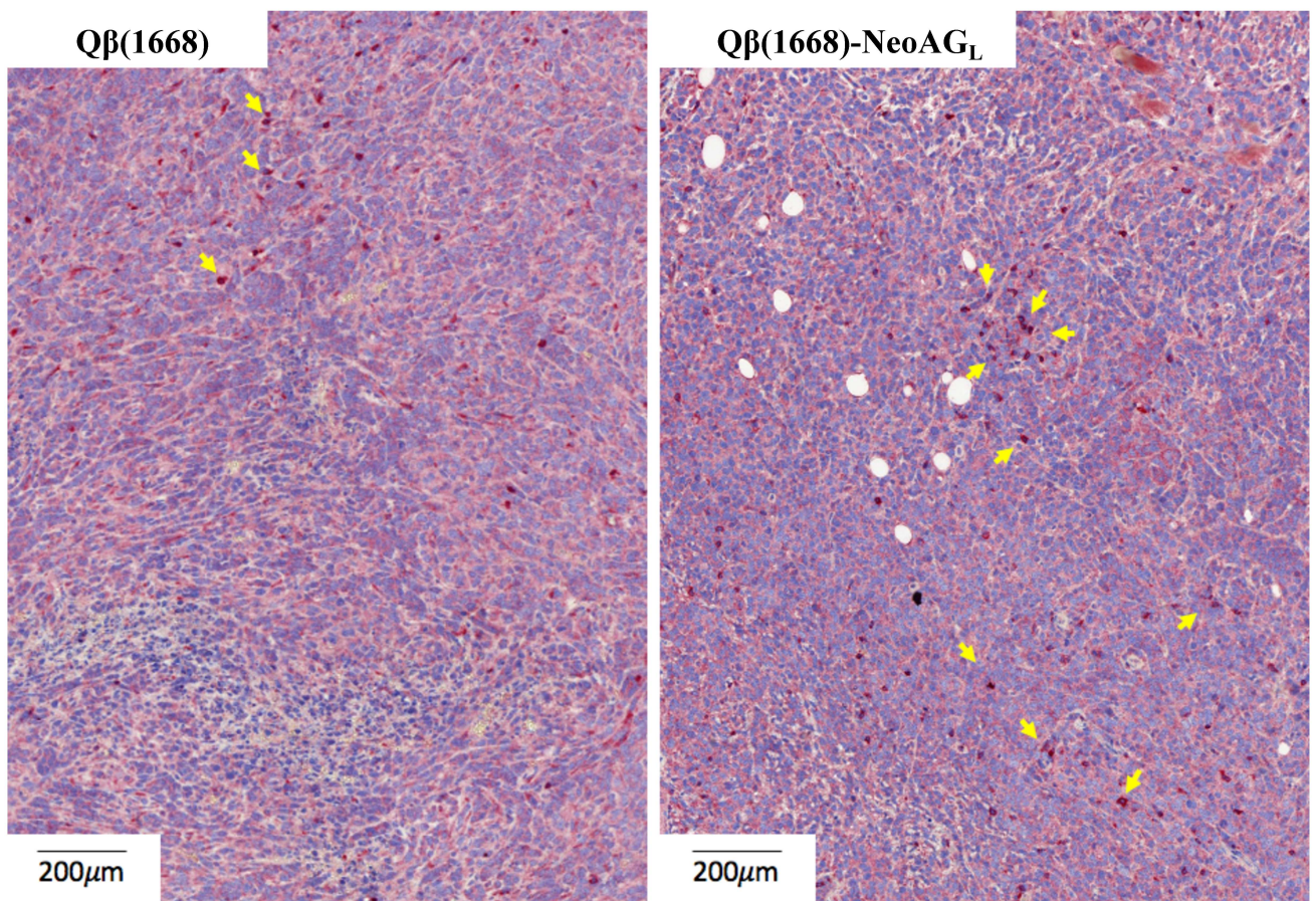
Supplementary Figure 4. Representative immunohistochemistry staining of CD4 + T cell for tumours treated with Q \beta (1668) as a control or Q \beta (1668)-NeoAG L . Arrows point to intratumoural CD4 + T cell. 3 samples per group were analysed.
