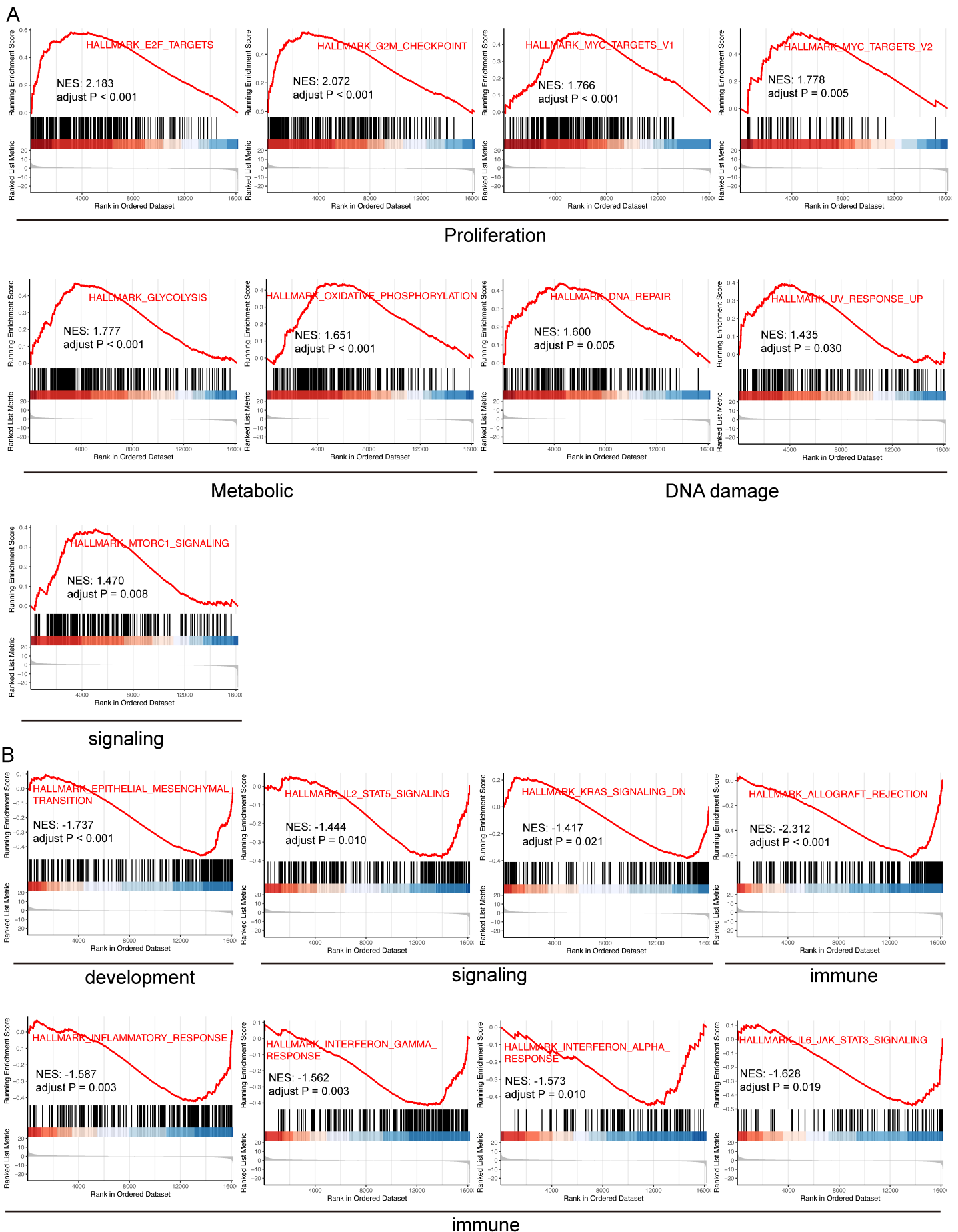
Figure S2. GSEA based on hallmark gene sets between brain metastases and primary LUAD. A . GSEA of brain metastases using hallmark gene sets; B . GSEA of primary LUAD using hallmark gene sets.
