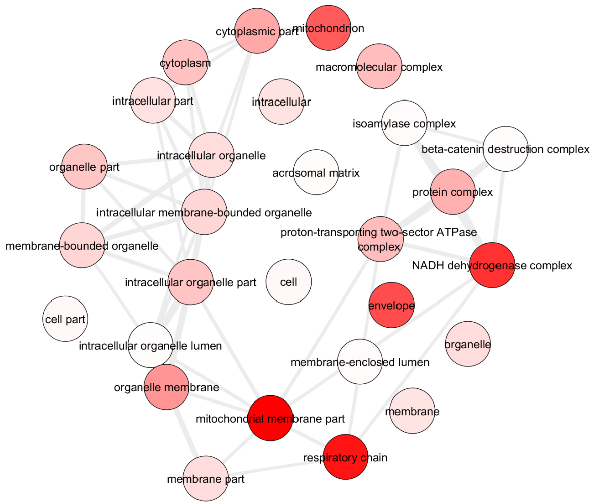
Figure S6. GO enrichment analysis for cellular components. REVIGO-generated network depicting relationships and overlap among significantly enriched cellular components. Enrichment score is indicated by color (darker red indicates greater enrichment).
