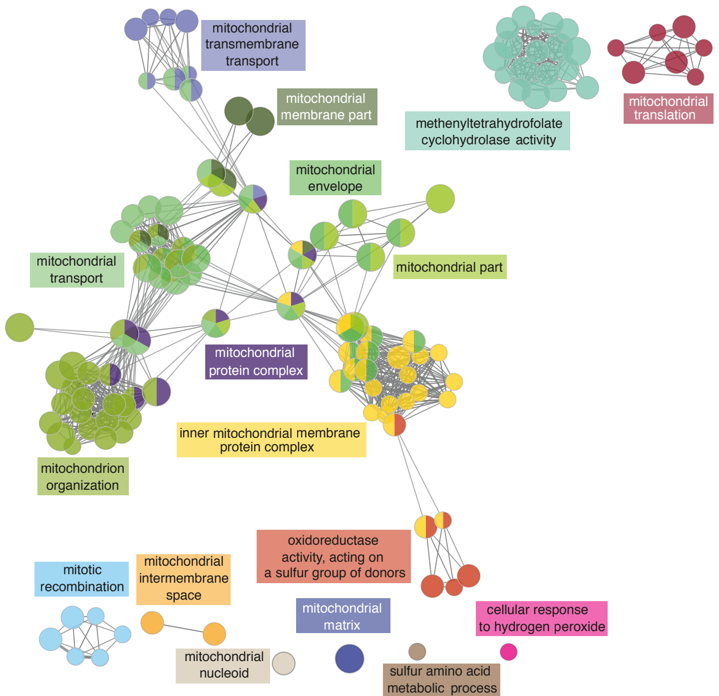
Figure S7. PD-1 targets different mitochondrial pathways and GO categories. ClueGo plot of the 84 mitochondrial genes differentially expressed in T_{ACT} and T_{ACT+PD1} cells. ClueGO visualizes the selected terms in a functionally grouped annotation network that reflects the relationships between the terms based on the similarity of their associated genes. The size of the nodes reflects the statistical significance of the terms. The group leading term for each cluster is indicated.
