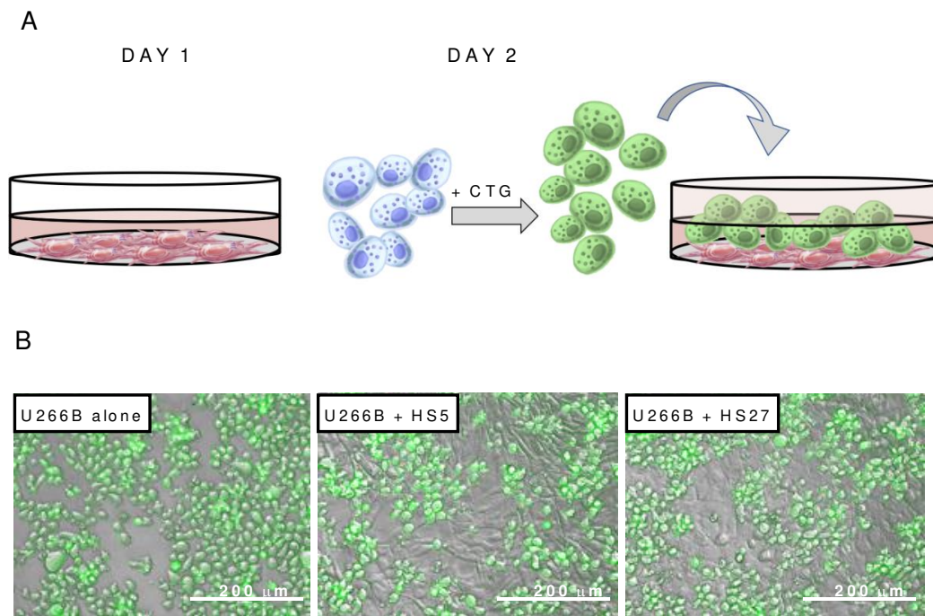
Supplementary Figure 1: MM:BMSC co-cultures. A) On Day 1, stromal cells (HS-5 or HS-27) were seeded and allowed to adhere. On Day 2, MM cells were stained with Cell Tracker Green (CTG) and added to stromal cells at a 1:1 ratio. Any medium already in the culture wells (conditioned by the stromal cells) was diluted 1:1 with fresh medium upon the addition of MM cells. B) Representative images of U266B cells cultured alone, or together with HS-5, or HS-27 stromal cells, respectively. Images taken using an EVOS® FL Cell Imaging System after a 24 hrs co-culture (ThermoFisher Scientific).
