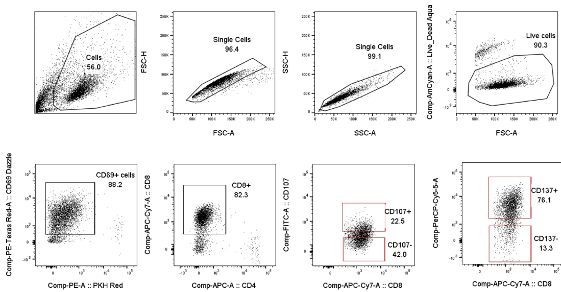
Fig. S9: Gating strategy used for the isolation of populations of CD107a pos , CD107a neg , CD137 pos , and CD137 neg CAR T cells subsequent to incubation with NALM-6 tumor cells. The sorted cells were subsequently used for RNA-seq.
