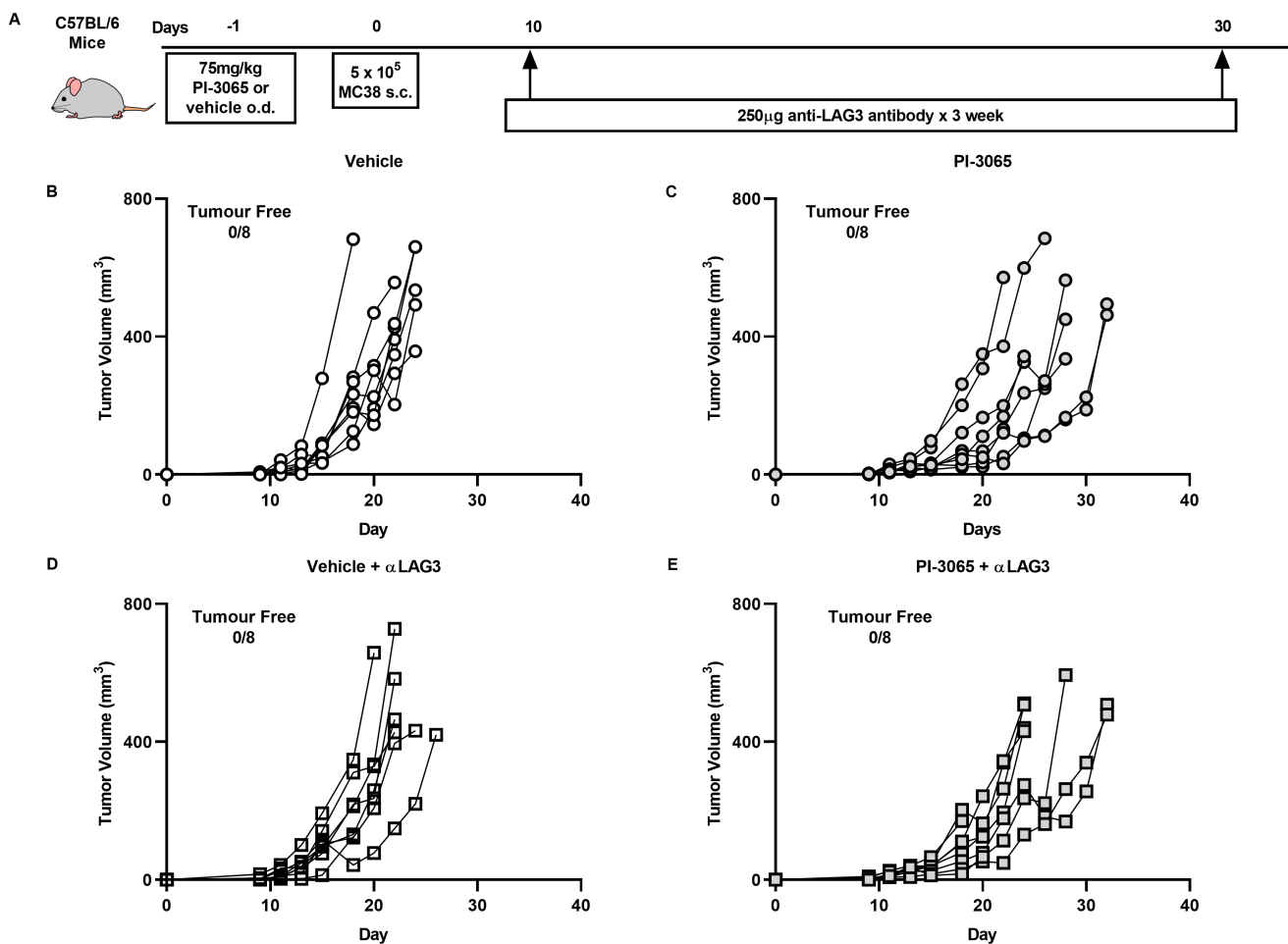
Supplementary Figure 2: Successful PI3K \delta combination therapy is tumour model dependent. (A) Schematic diagram shows the experimental protocol: MC38 mice were treated daily for the duration of the study with either 75mg/kg of PI-3065 or vehicle by oral gavage and were administered anti-LAG3 (250µg) at the days indicated (8 mice/group). Individual growth curves from MC38 tumour bearing mice treated with (B) vehicle (C) PI-3065 (D) vehicle + anti-LAG3 or (E) PI-3065 + anti-LAG3.
