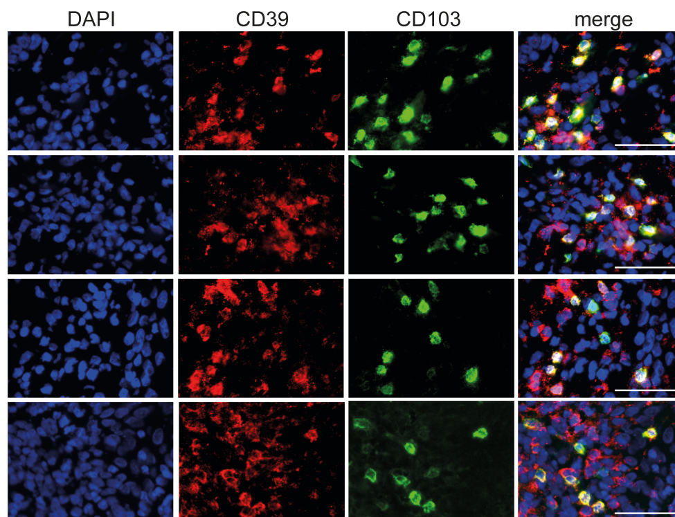
Supplementary Figure 6. Expression of CD39 by CD103+ T cells in cSCC. Representative immunofluorescence microscopy images of cSCC stained for CD103 and CD39. Scale bars = 50 \mu m.
