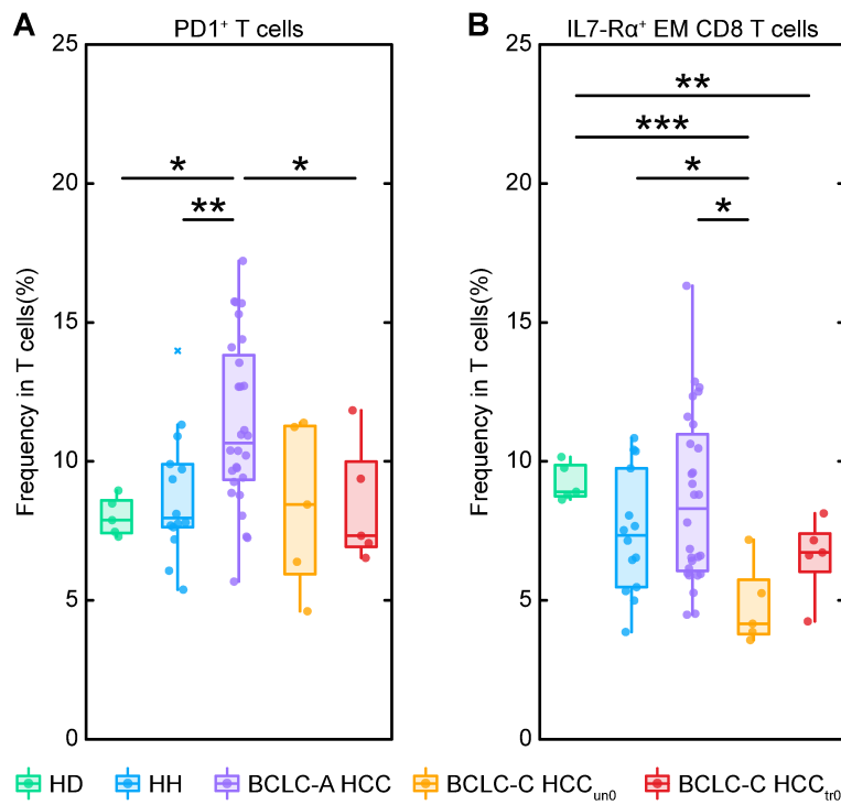
Supplementary Figure 5. Comparisons of selected immune subsets across HD, HH, and HCC groups.
